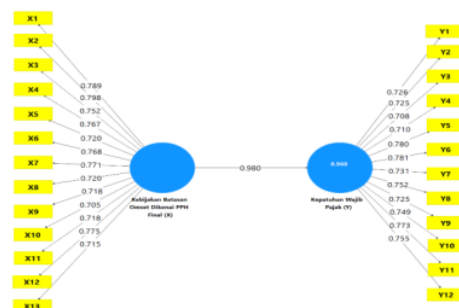
Picture 1. Path Diagram
