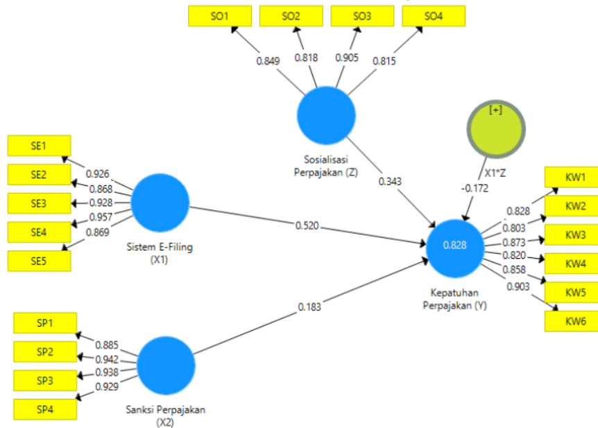
Figure 2. Path Diagram
