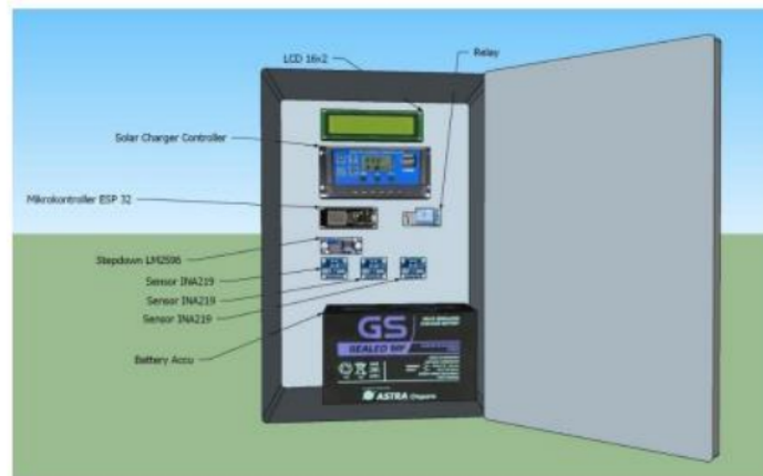
Gambar 3. Gambar Desain Box Panel
