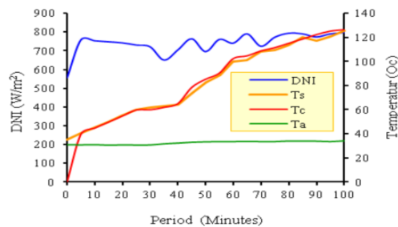
Fig. 9. Relationship of DNI, T_s , T_c , T_a versus tracker movement period every 5 minutes
