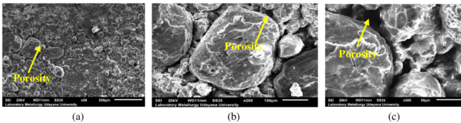
Figure 11. SEM photo of composition II at a temperature of 550°C with (a) 50x; (b) 200x; (c) 500x magnification
