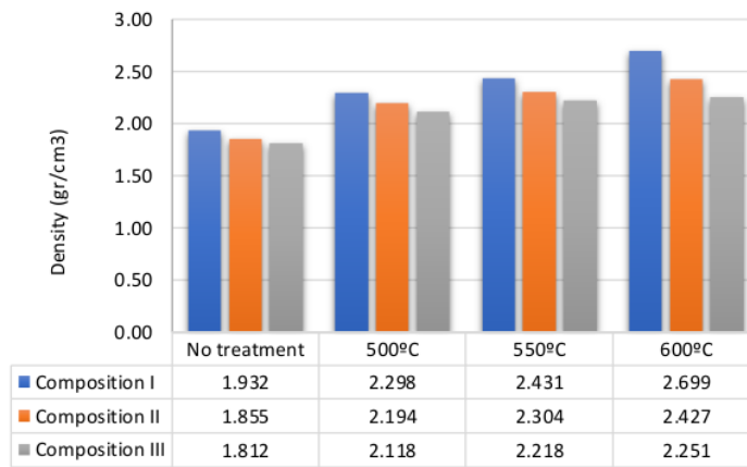
Figure 6. Graph of composite density results on the composition against temperature and without treatment
