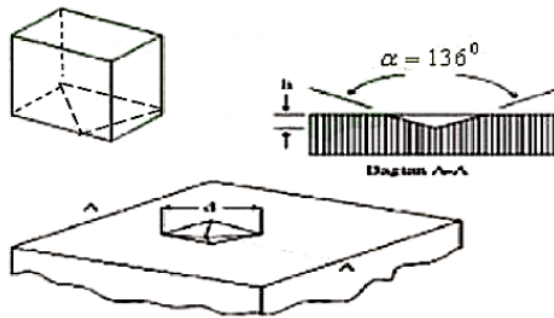
Figure 1. Hardness testing schematic
