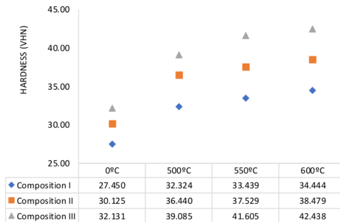
Figure 8. Graph of composite hardness test results against temperature treatment
