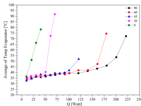
17 Figure 4 Effect of inclination angle on the range of OHP working temperature
