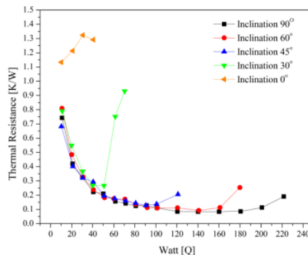
Figure 6 Thermal Resistance at different inclinations
