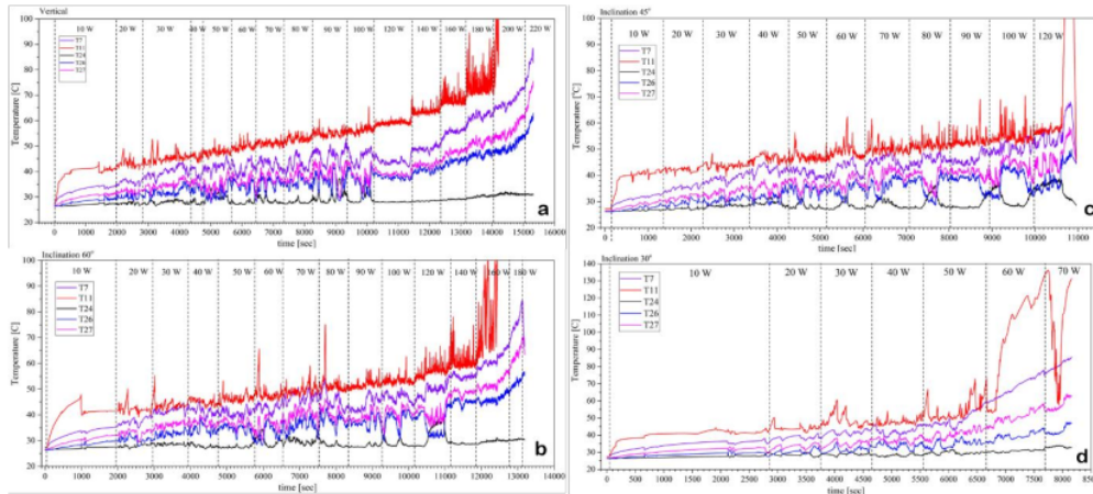
Figure 2 Effect of inclination for temperature fluctuations at: (a) Inclination of 90^\circ ; (b) Inclination of 60^\circ ; (c) Inclination of 45^\circ ; and (d) Inclination of 30^\circ
