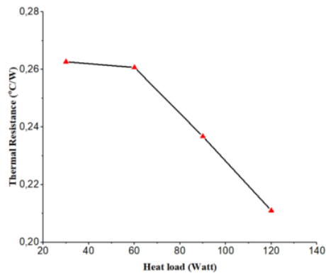
Figure 7. The thermal resistance of PHP.
