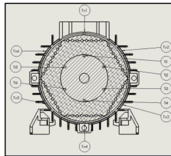
Figure 2. Thermocouple placement.
