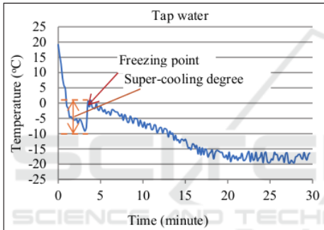
Figure 2: Cooling process and super-cooling tap water.
