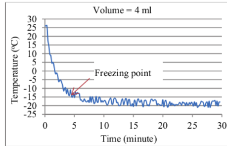
Figure 4: Cooling process and Jatropa oil freezing point for sample 4 ml.
