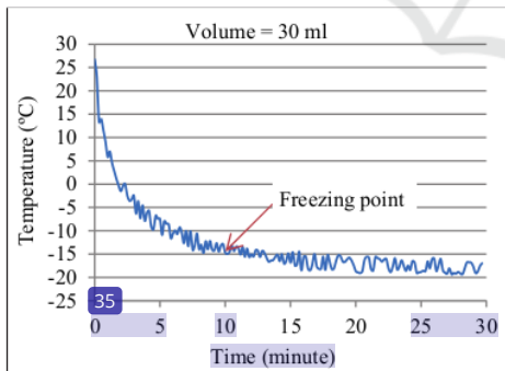
Figure 9: Cooling process and Jatropa oil freezing point for sample 30 ml.
