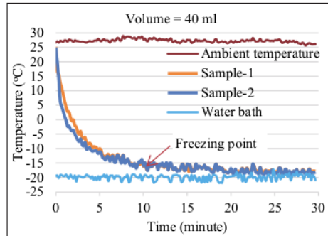
Figure 10: Cooling process and Jatropa oil freezing point for sample 40 ml.
