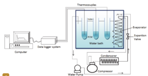
6 Figure 1: Schematic diagram of the experimental test equipment T-history method (Rasta, et al., 2016a).
