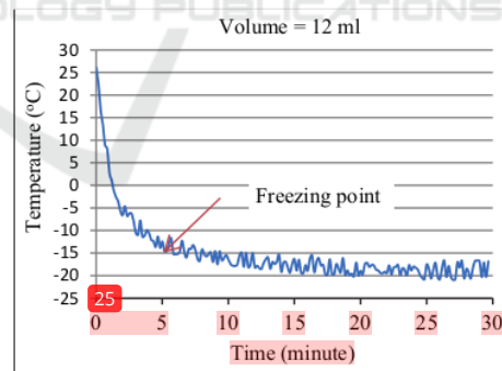
Figure 6: Cooling process and Jatropa oil freezing point for sample 12 ml.
