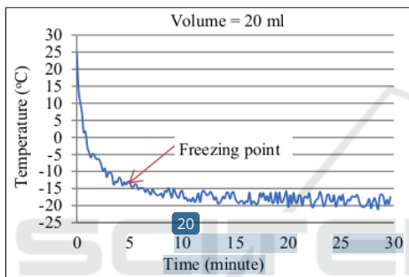
Figure 8: Cooling process and Jatropa oil freezing point for sample 20 ml.
