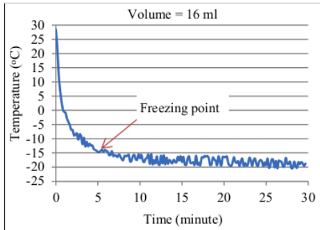
Figure 7: Cooling process and Jatropa oil freezing point for sample 16 ml.
