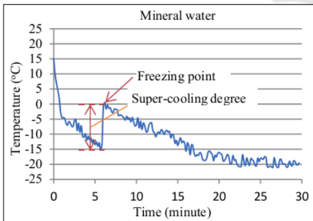
Figure 3: Cooling process and super-cooling mineral water.
