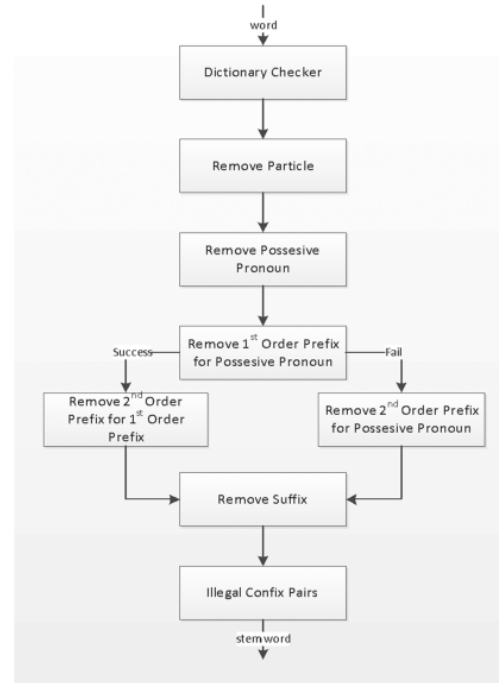
Fig. 2. Stemming process.
