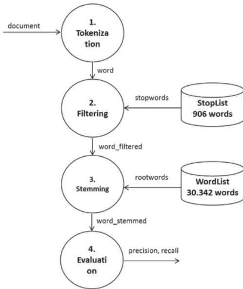
Fig. 1. Text processing application architecture.
