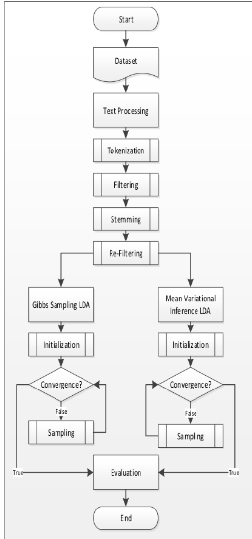
Fig. 1. Algorithm of Gibbs Sampling LDA
