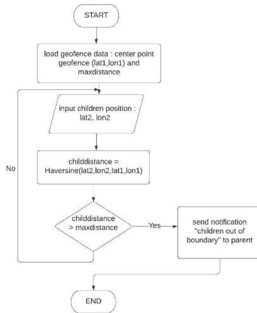
Figure 3. Flowchart for Circular Shape Geofence Detection
