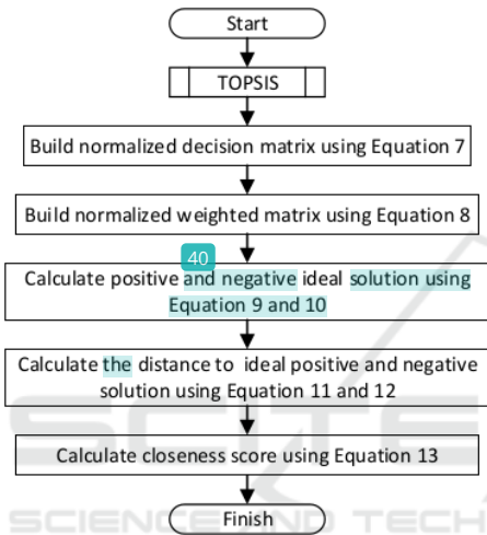
Figure 3: The flowchart of TOPSIS.
