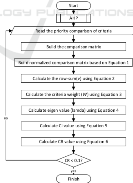
Figure 2: The flowchart of AHP.
