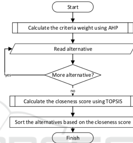
Figure 1: The combination of AHP and TOPSIS.
