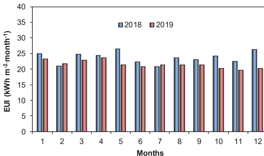
Fig. 12. Energy use intensity (EUI) of the hotel for two-year period
