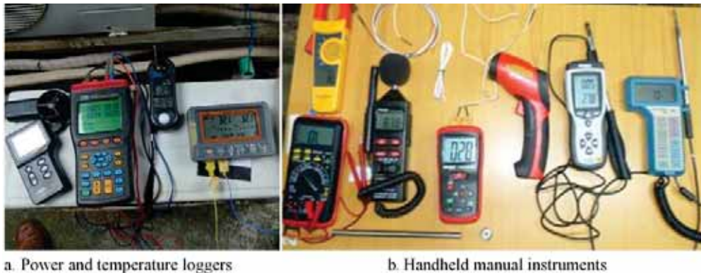
Fig. 7. Handheld instruments for automatic and manual measurements
