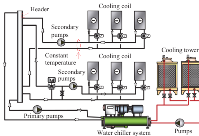
Figure 2. Air conditioning system with water cooled chillers
