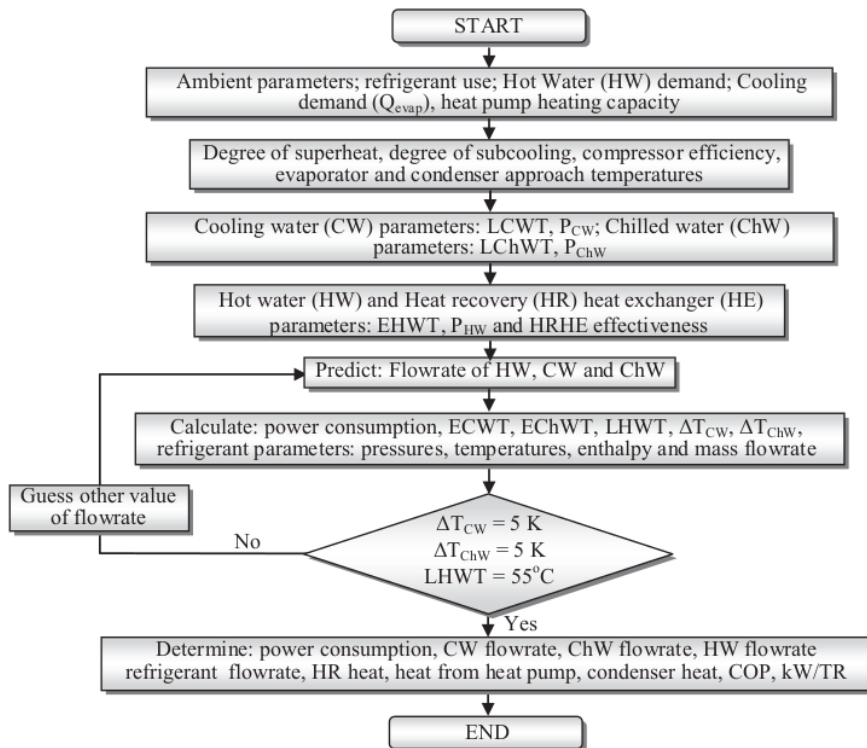
Figure 1. Structure of the EES simulation models for integrated heat recovery AC system and heat pump
