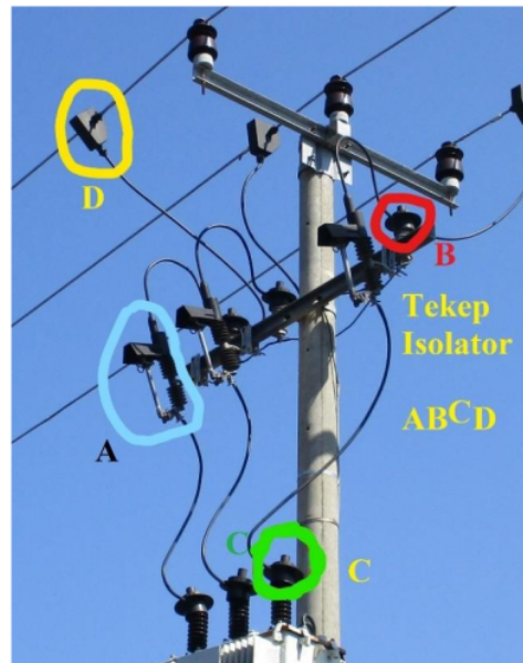
Gambar 4 Tekep isolator gardu: FCO (A), arrester (B), bushing (C), connector (D).
