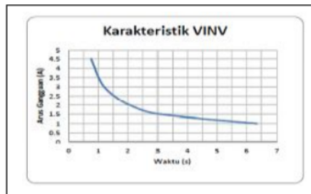
Gambar 11.Karakteristik waktu Very Inverse
