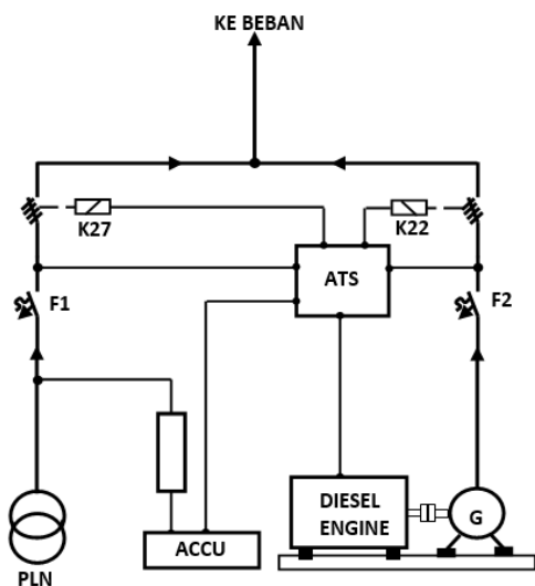
Gambar 2. Diagram balok sistem power supply .
