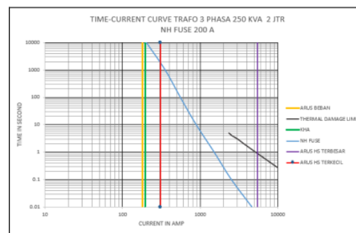
Gambar 17. Grafik time current curve DB0575
