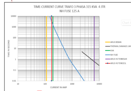
Gambar 16. Grafik time current curve DB0292
