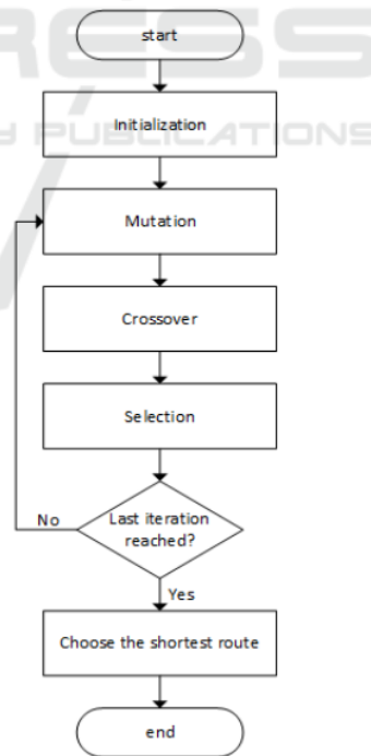
Figure 1: Flowchart of routing with differential evolution.
