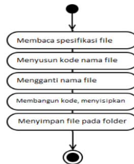
Gambar 2. Activity Diagram Simpan File
