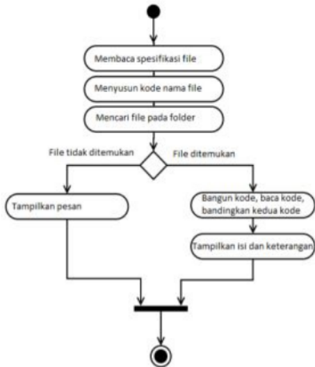
Gambar 3. Activity Diagram Cari File
