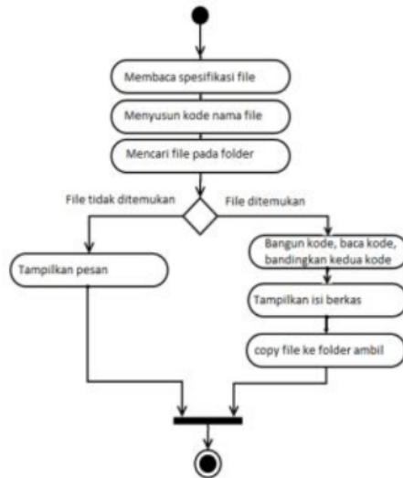
Gambar 4. Activity Diagram Ambil File
