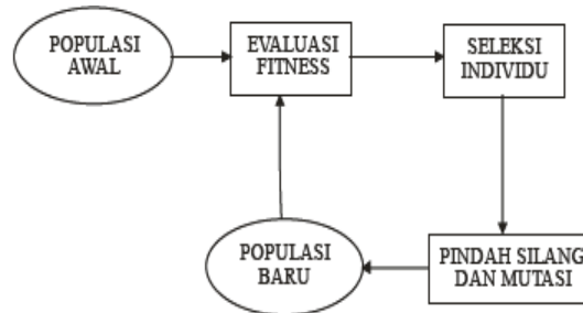
Figure 1. Cycle of genetics algorithm
