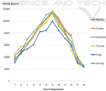
Figure 7: Curve of polar panel intensity average.
