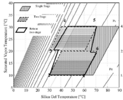
Gambar 2. Diagram P-T-X dari Re-Heat Two-Stage Chiller
