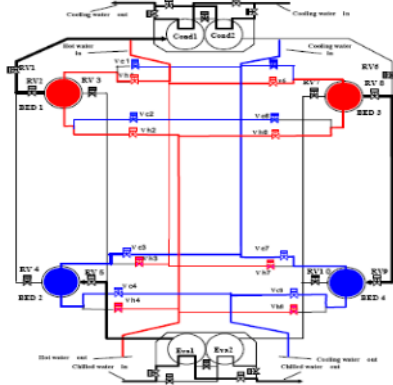
Gambar 1. Four-Bed Reheat Adsorption Cycle Scheme
