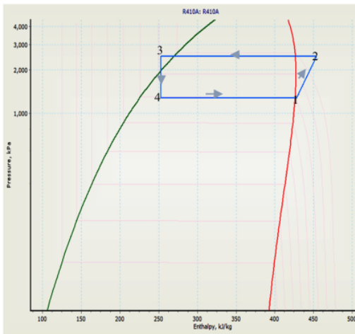
Figure 2. P-h diagram of system with R410a
