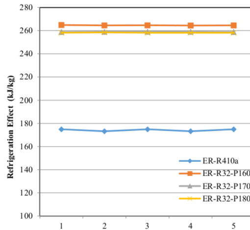
Figure 4. Refrigerant Effects of R410a and R32 Refrigerants
