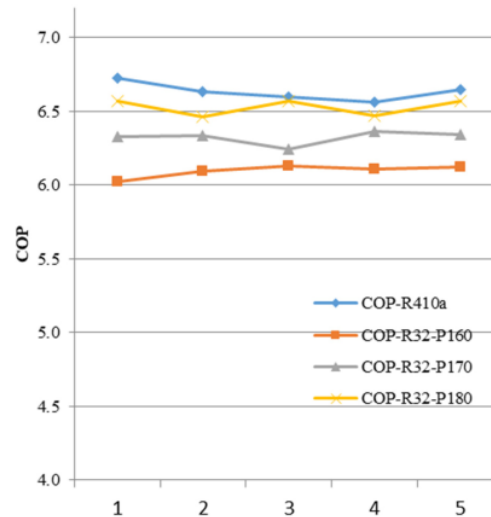
Figure 5. COP system with R410a and R32 refrigerants
