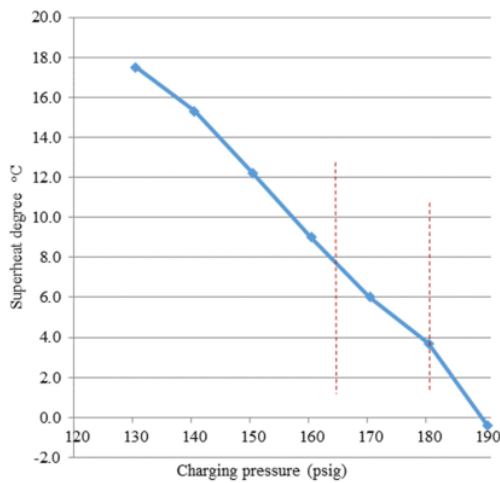
Figure 3. R32 superheat degree at various charging pressure
