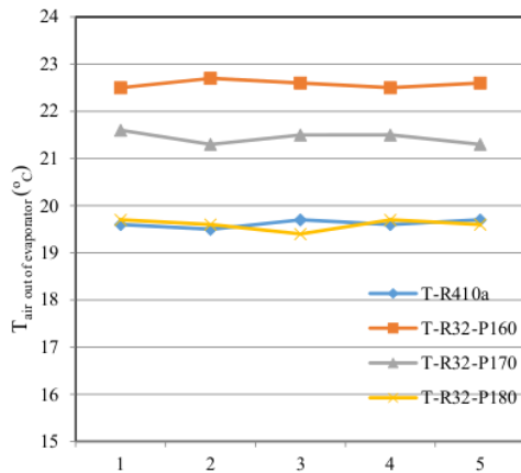
Figure 6. Temperature of air out evaporator
