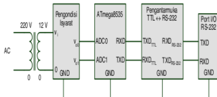
Gambar 1 Blok diagram system
