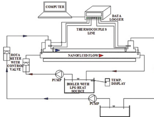
Fig. 1. Experiment apparatus set-up.
