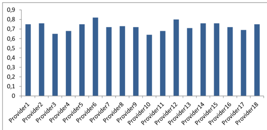
Figure 3. The final score of all providers
