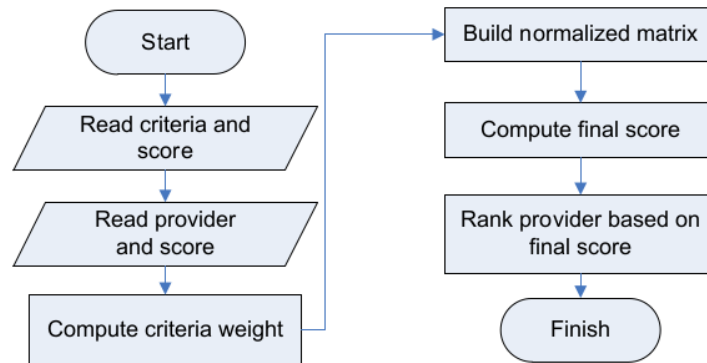
Figure 1. The flowchart of SAW
