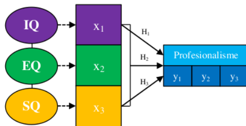
Fig. 1. Model Of Variable, Indicators and hipotesis
